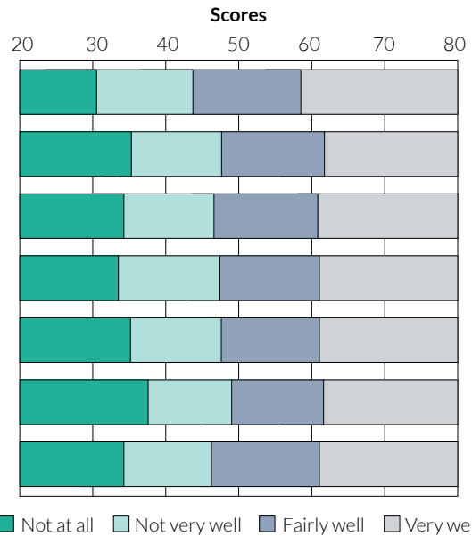
Figure A.2: Item map for the scale reflecting students' citizenship self-efficacy
